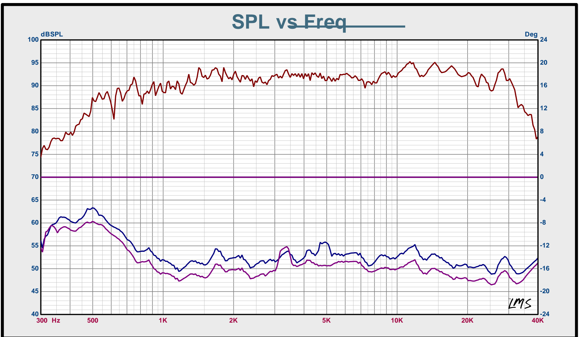
Fig 2. SPL(Red, 1m*1w) Curve
