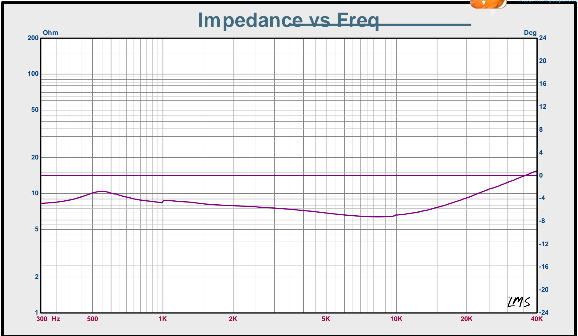
Fig 1. Impedance
